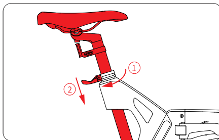
5. When installing the saddle, rotate the fixed latch①outward to open, and then insert the saddle ② into the seat tube.
