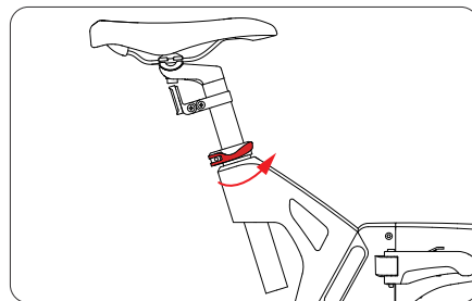
6. Rotate the latch in the indicated direction to tighten it. Please check that the saddle does not roll back or shake when pressed.
